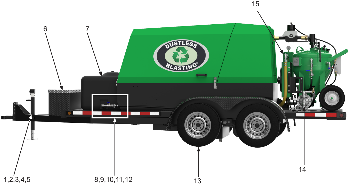
Figure 2: Dustless Blasting DB500 Mobile S Pro Blaster
